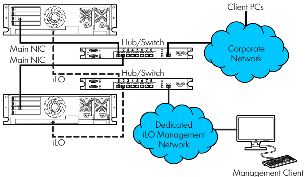
Figure 2 Dedicated management network diagram
