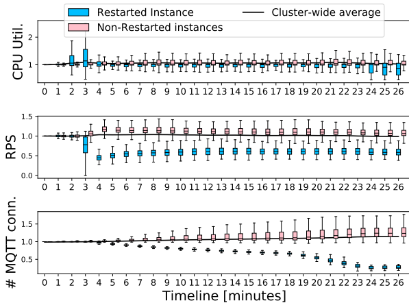
Figure (13) Timeline of Proxygen restart
